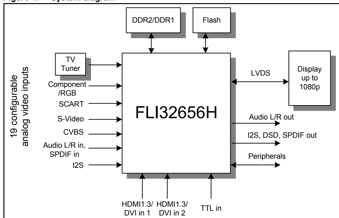
Figure 1. System diagram
