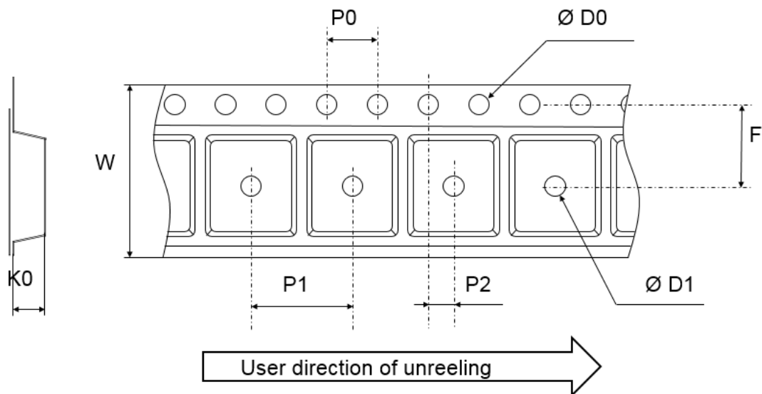
Figure 22. Tape outline
