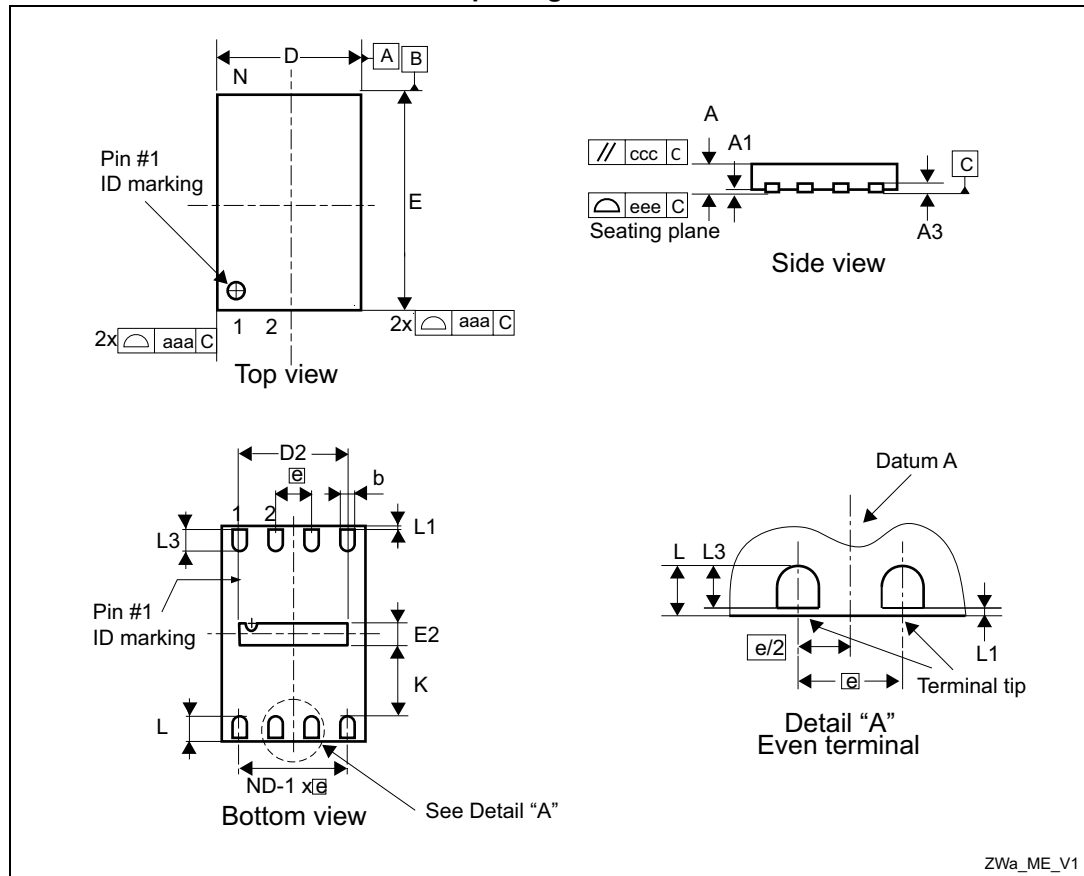
Figure 21. UFDFPN8 - 8-lead, 2 × 3 mm, 0.5 mm pitch ultra thin profile fine pitch dual flat package outline
