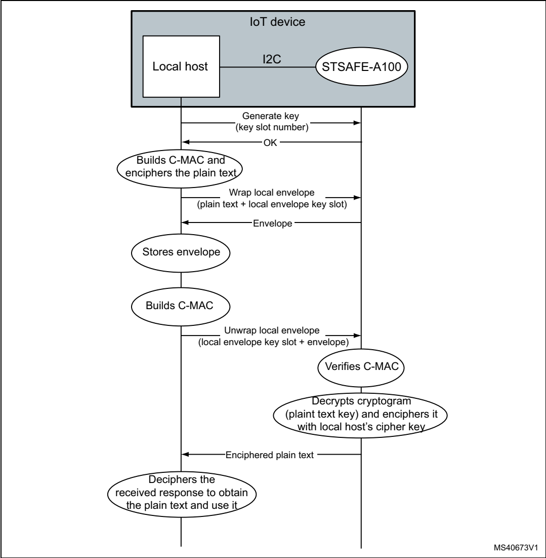
Figure 15. Wrap/Unwrap Local Envelop command flow
