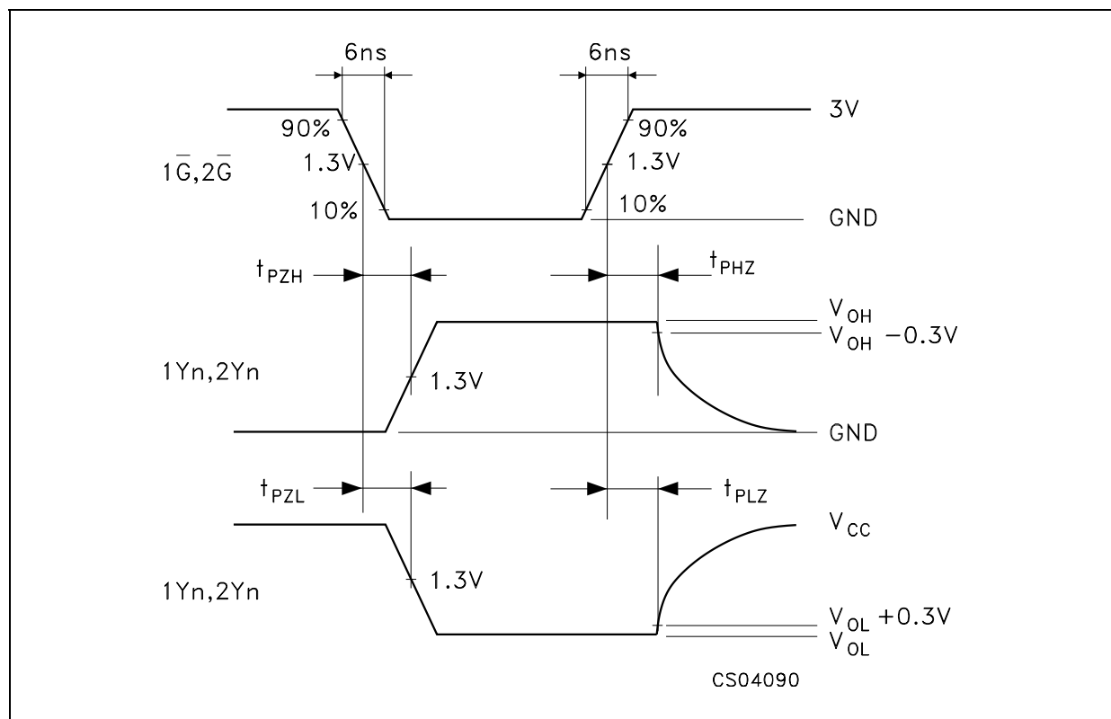
Figure 4: Waveform - Output And Enable Times ( f=1\text{MHz} ; 50% duty cycle)
