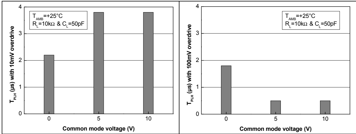
Figure 9. T_{PLH} vs V_{icm} at V_{CC} = 5\text{ V} and 10 mV overdrive Figure 10. T_{PLH} vs V_{icm} at V_{CC} = 5\text{ V} and 100 mV overdrive
