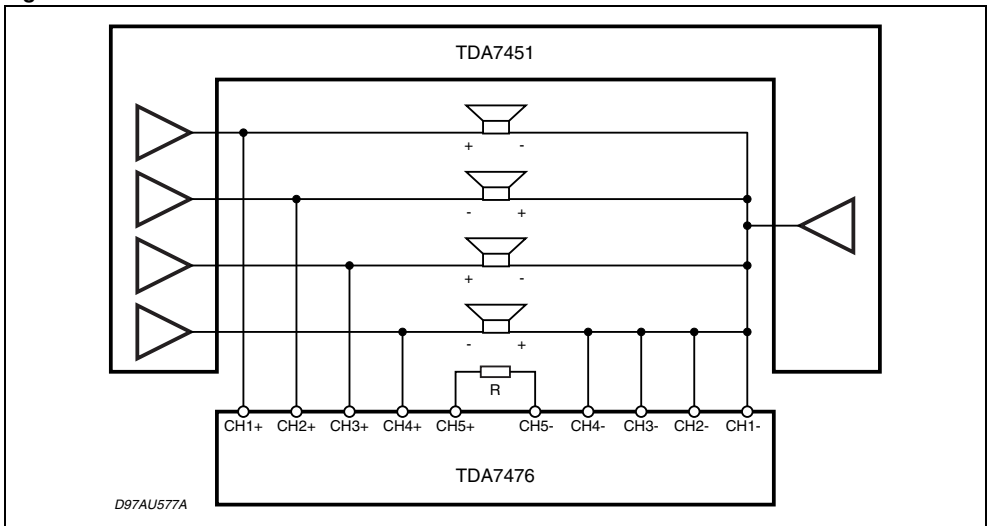
Figure 6. TDA7451
