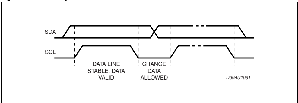
Figure 2. Data Validity on the I 2 C BUS
