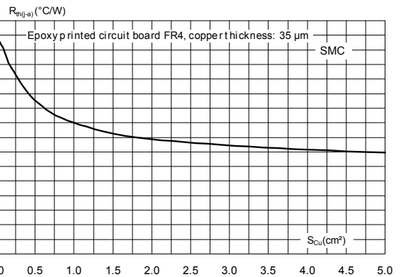
Figure 12. Thermal resistance junction to ambient versus copper surface under each lead (SMC)
