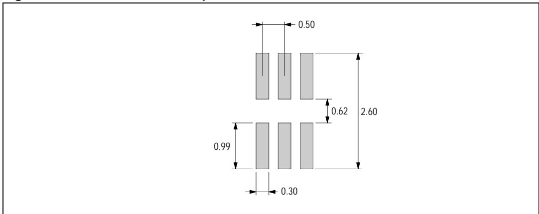
Figure 17. Recommended footprint
