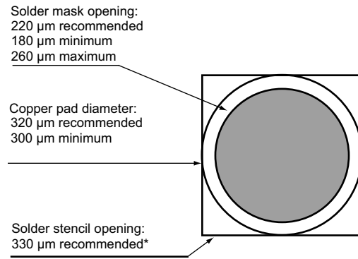
Figure 18. Footprint - 5 mils stencil - solder mask defined
