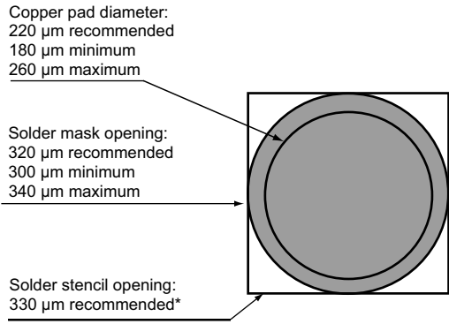
Figure 17. Footprint - 5 mils stencil - non solder mask defined
