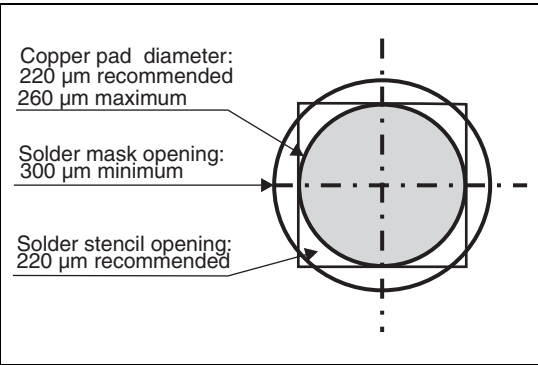
Figure 18. Footprint
