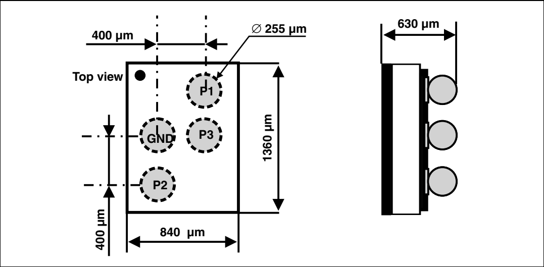
Figure 17. Package dimensions
