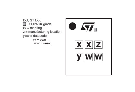
Figure 19. Marking
