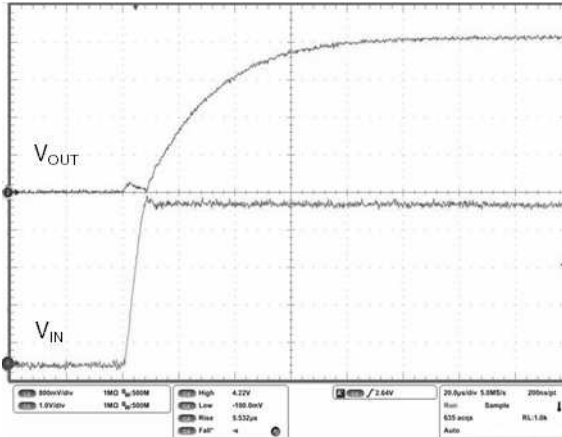
Figure 30. Startup transient
