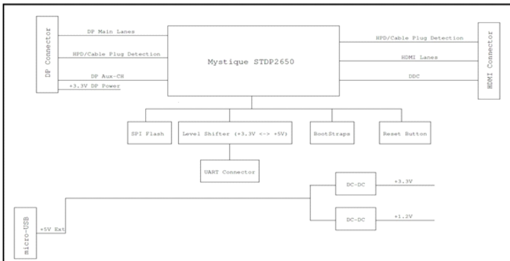
Figure 3. Connection diagram
