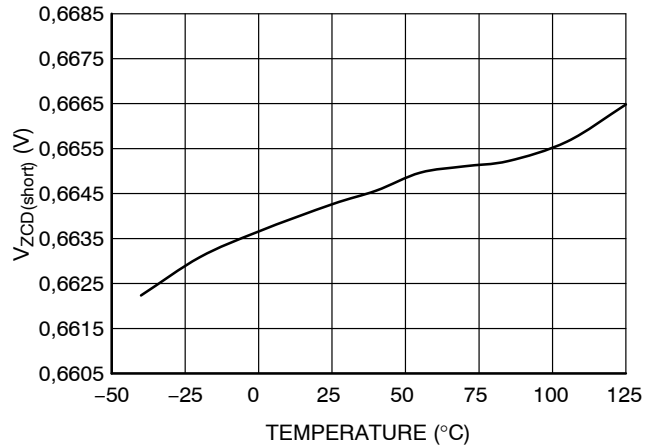
Figure 30. V_{ZCD(short)} vs. Temperature
