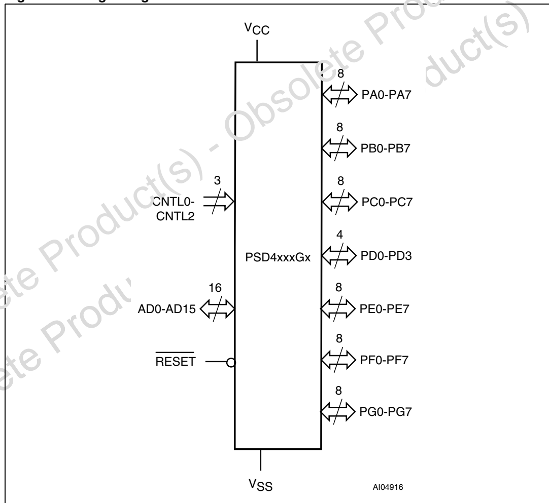
Figure 2. Logic diagram
