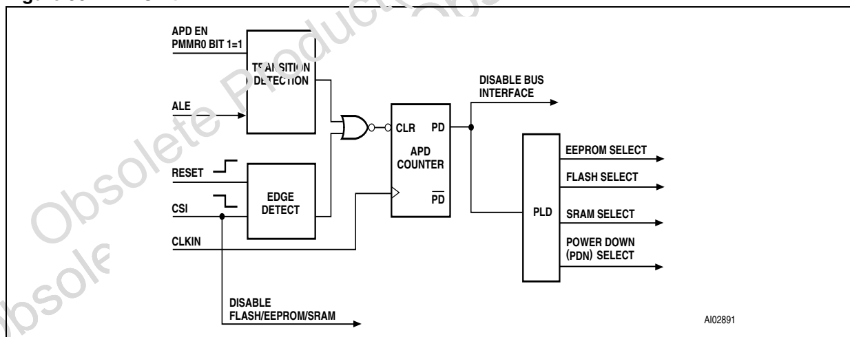
Figure 33. APD Unit
