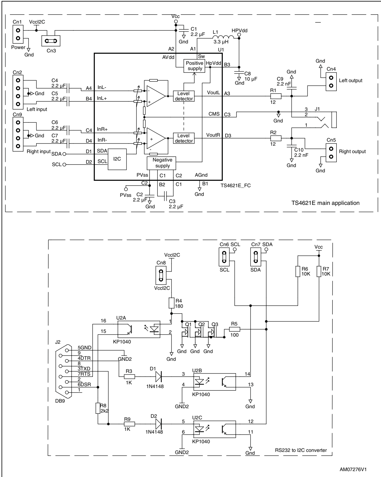
Figure 1. Circuit schematics
