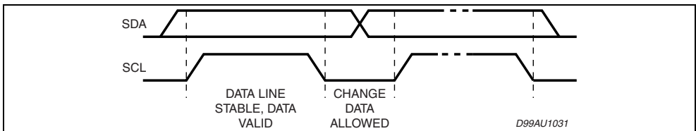
Figure 17. Timing Diagram on the I 2 C BUS
