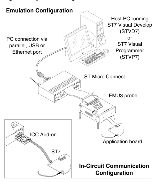
Figure 1: System configurations
