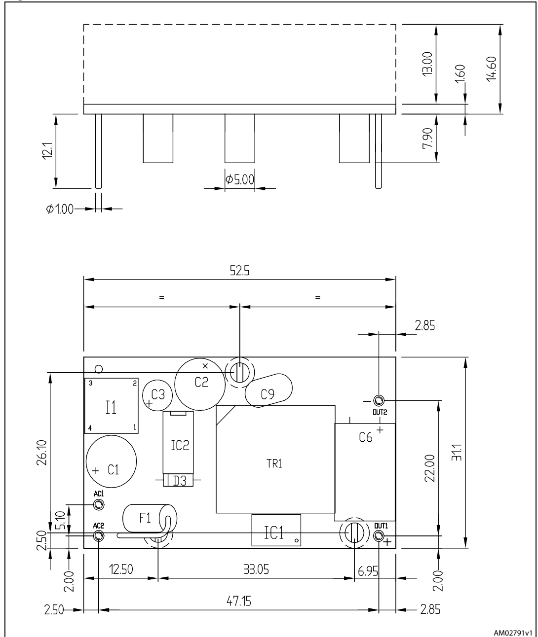
Figure 1. Pin connection
