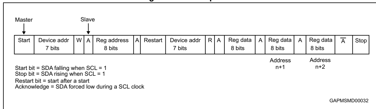
Figure 11. Read operation
