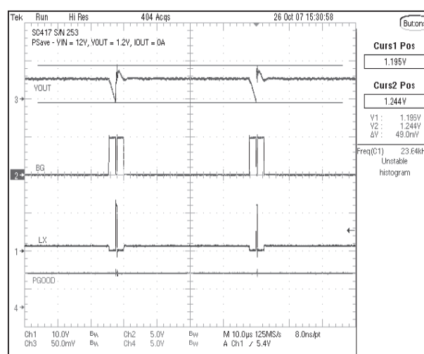
Figure 6 - Ultrasonic Power-Save Operation Mode
