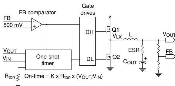
Figure 2 - On-Time Generation
