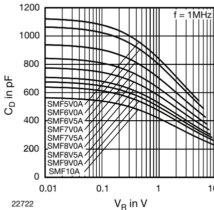
Fig. 8 - Typical Capacitance C_D vs. Reverse Voltage V_R
