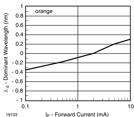
Fig. 4 - Dominant Wavelength vs. Forward Current
