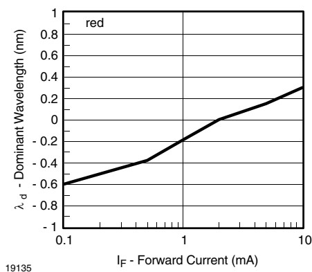
Fig. 16 - Dominant Wavelength vs. Forward Current
