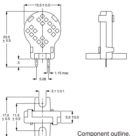
Component outline.
