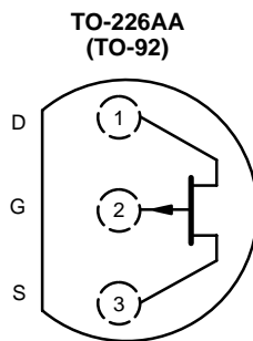
Top View J270 J271
