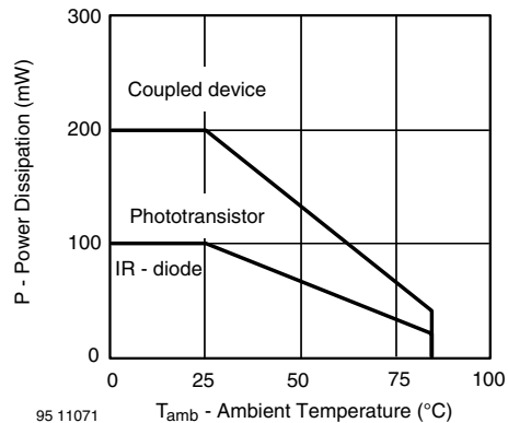
Figure 1. Power Dissipation Limit vs. Ambient Temperature
