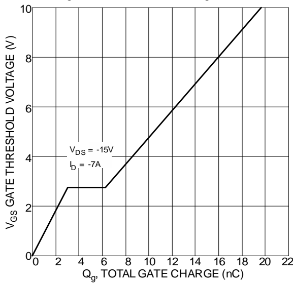
Figure 23 Gate Charge
