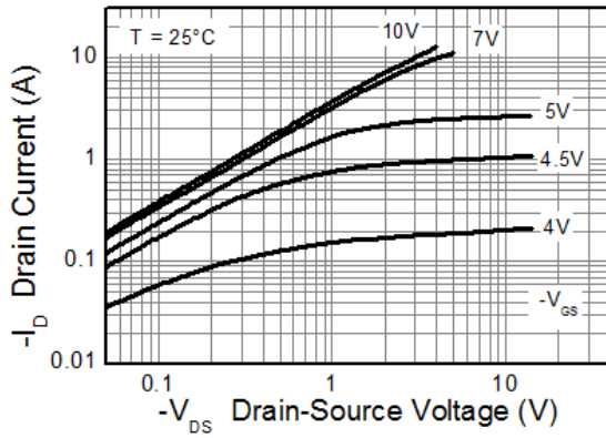
Output Characteristics
