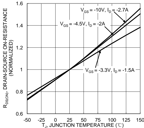
Figure 18. On-Resistance Variation with Junction Temperature
