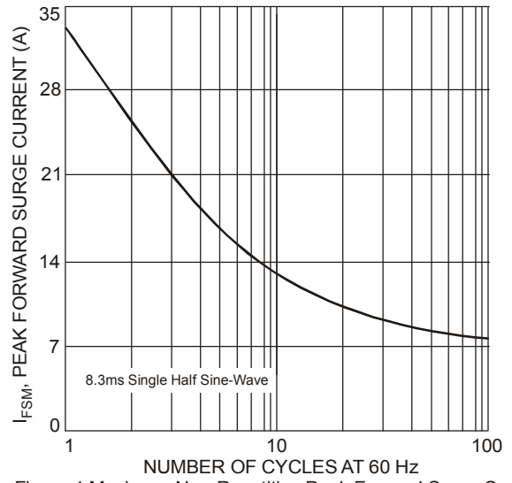
Figure 4 Maximum Non-Repetitive Peak Forward Surge Current
