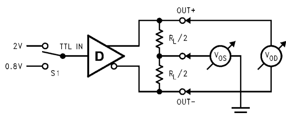
FIGURE 1. Differential Driver DC Test Circuit
