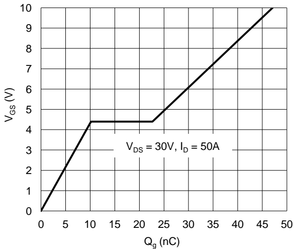
Figure 11. Gate Charge
