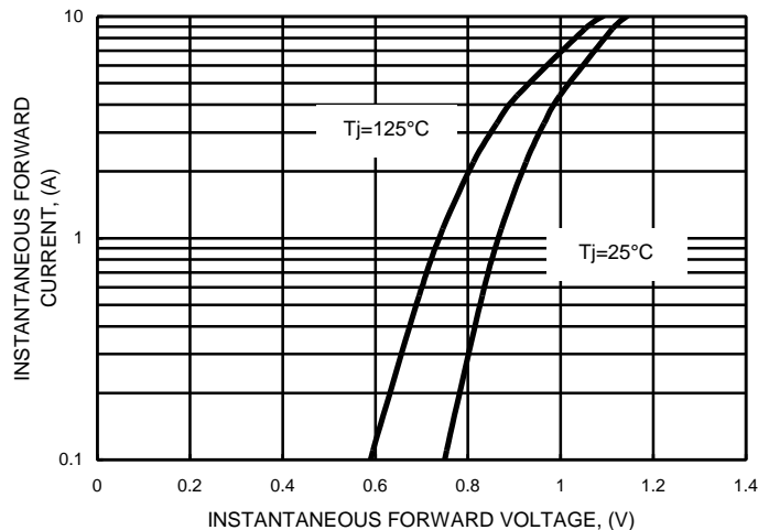
FIG.3- TYPICAL FOWRD CHARACTERISTICS
