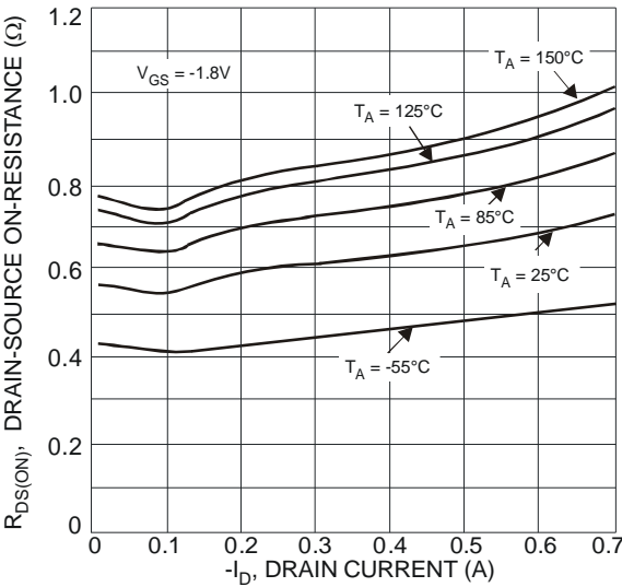
Fig. 8 Typical On-Resistance vs. Drain Current and Temperature
