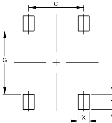
T-DFN5564-4
