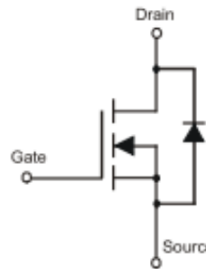
Equivalent Circuit
