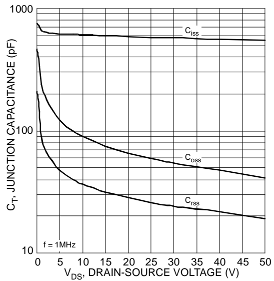
Figure 10 Typical Junction Capacitance
