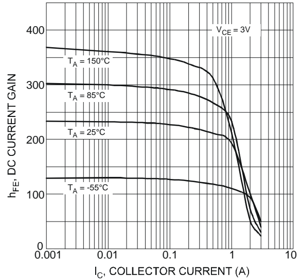
Figure 2. Typical DC Current Gain vs. Collector Current (2DD1664R)
