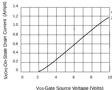
Transfer Characteristics
