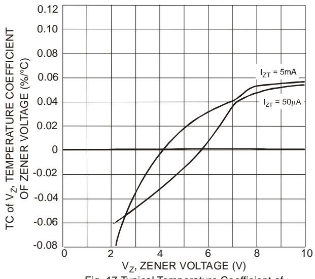
Fig. 17 Typical Temperature Coefficient of Zener Voltage vs. Zener Voltage, DDZ9681 - DDZ9697
