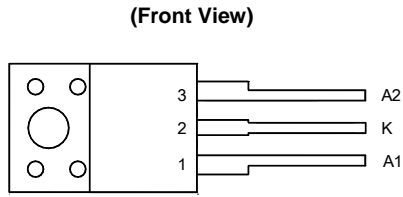
TO-220F-3 (Option 1)
