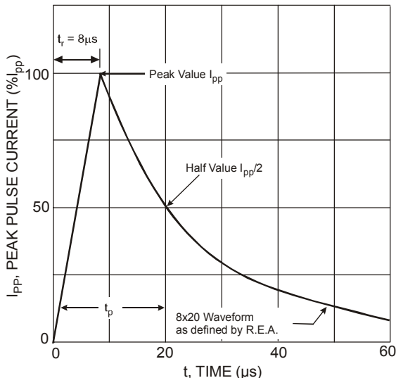
Figure 1 Pulse Waveform
