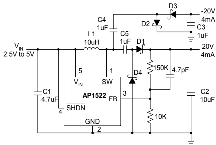
\pm 20V Dual Output Converter with Output Disconnect
