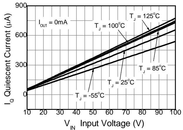
Quiescent Current
