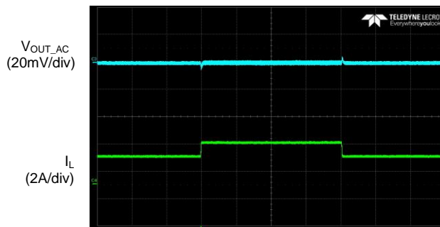
Load Transient (I OUT =2A to 3A)
