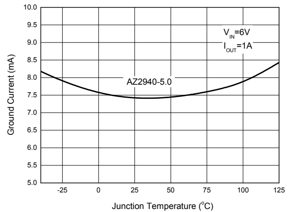
Figure 11. Ground Current vs. Junction Temperature
