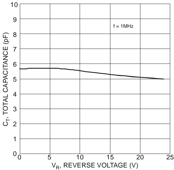
Figure 5 Typical Capacitance
