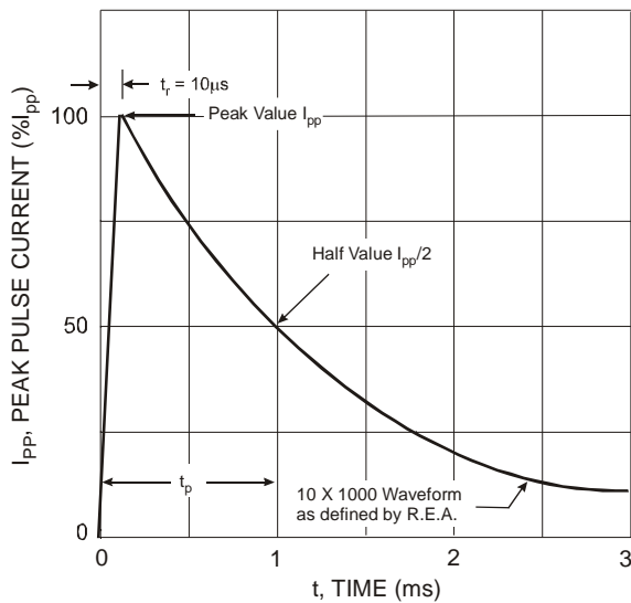
Figure 1 Pulse Waveform
