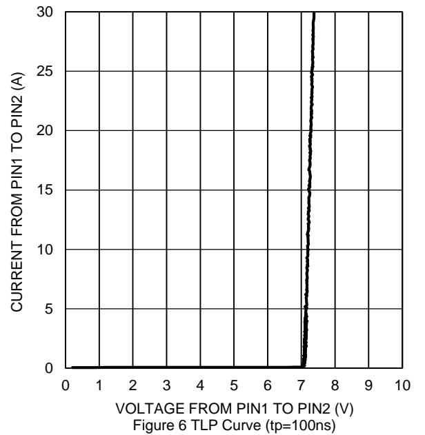
Figure 6 TLP Curve (tp=100ns)
