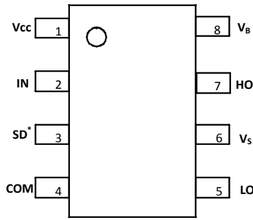
Top View: SO-8 (Type TH)
