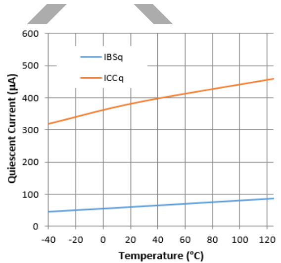
Figure 13. Quiescent Current vs. Temperature
