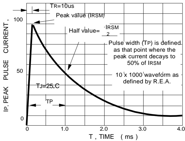
FIG.5 - PULSE WAVEFORM
